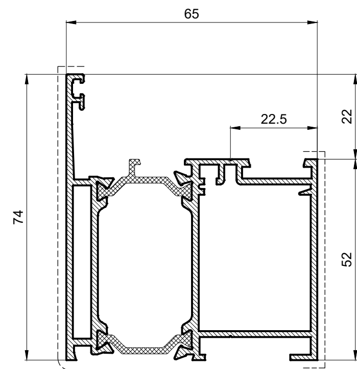
PR65106 1.760 Kg/m
