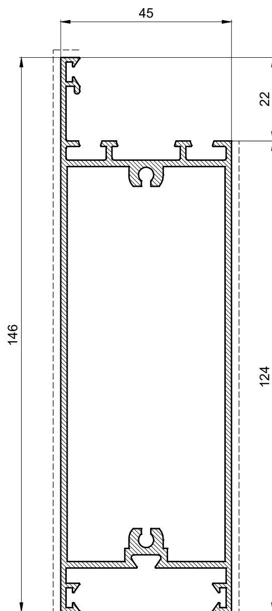
PM 40022 1,955 Kg/m
