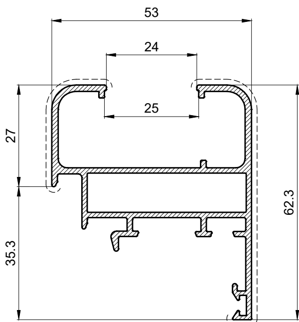
PM 40050 1,042 Kg/m
