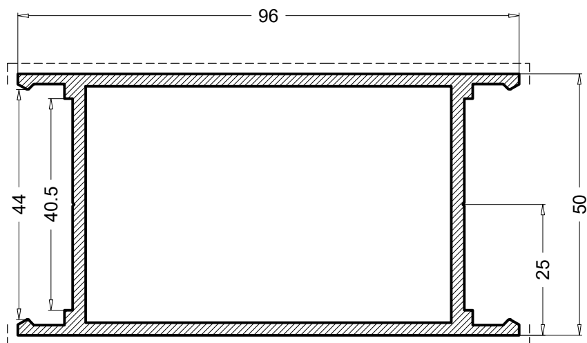
OE80130 1.871 Kg/m
