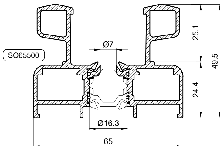
SECTION H-H
